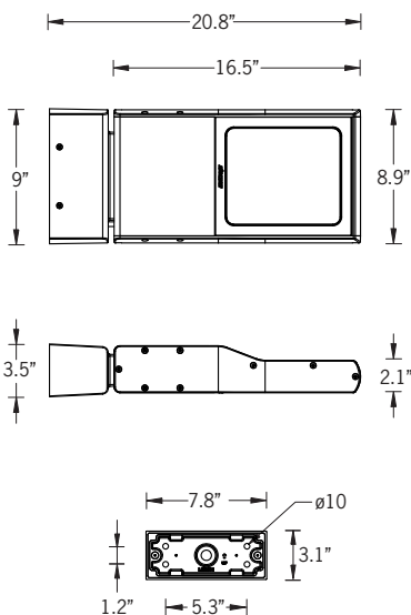
Mounting Detail
