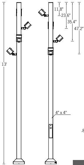
Mounting Detail
